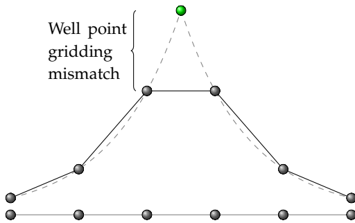
Figure 18.1. Vertical cross section of a surface. Grid nodes are marked as grey dots. A single well point is marked as a green dot. The dashed line is the kriging predictor and the solid line is the bilinear interpolation between the grid nodes. The gridding error is the vertical difference between the dashed line (kriging) and the solid line segments (bilinear interpolation). The gridding mismatch at a well point is the vertical difference between the green dot and the solid line connecting the two nearest grid nodes.
