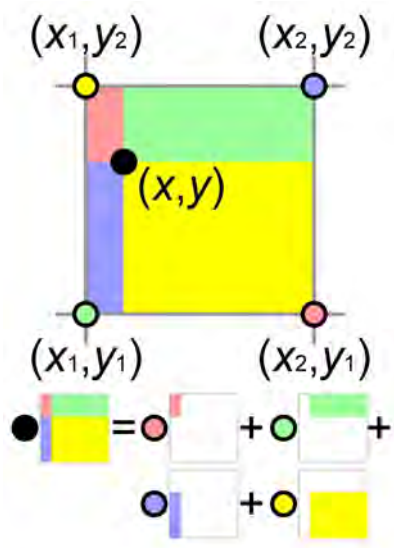
Figure 20.3. Illustration of bilinear interpolation. The value at the black dot, (x, y) , is the weighted average of the values at the colored dots, (x_i, y_j) ; i, j = 1, 2 , where the weights are proportional to the area of the rectangle of the same color. The illustration is taken from Wikipedia .
