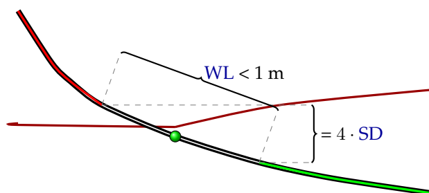
Figure 8.10. Cross section of one surface along a well path. A short ( \Delta WL \leq 1 meter) undefined zone log section is replaced by a well point (green dot) at the center with TVD pick uncertainty (SD) equal to \frac{1}{4} \Delta TVD .
