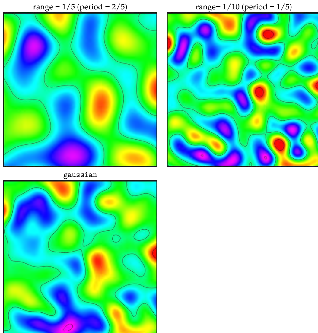
Figure 22.4. Simulated realization using damped sine variograms. The damped sine variogram gives a smooth regular cyclic appearance. The full period is twice the specified range. The gaussian variogram is added for comparison.
