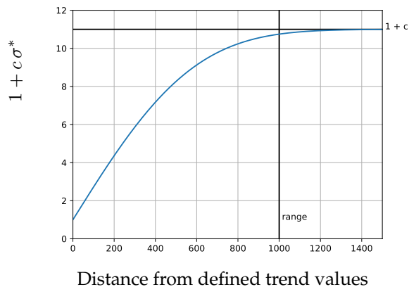
Figure 18.3. Increase in residual SD in areas with extrapolated trend maps. The default value c = 10 is used in the figure. The SD increases until it reaches the range given by <extrapolation-kriging-range> where it flattens at 1 + c times the original local SD value. The factor c is specified by <extrapolation-SD-factor>.
