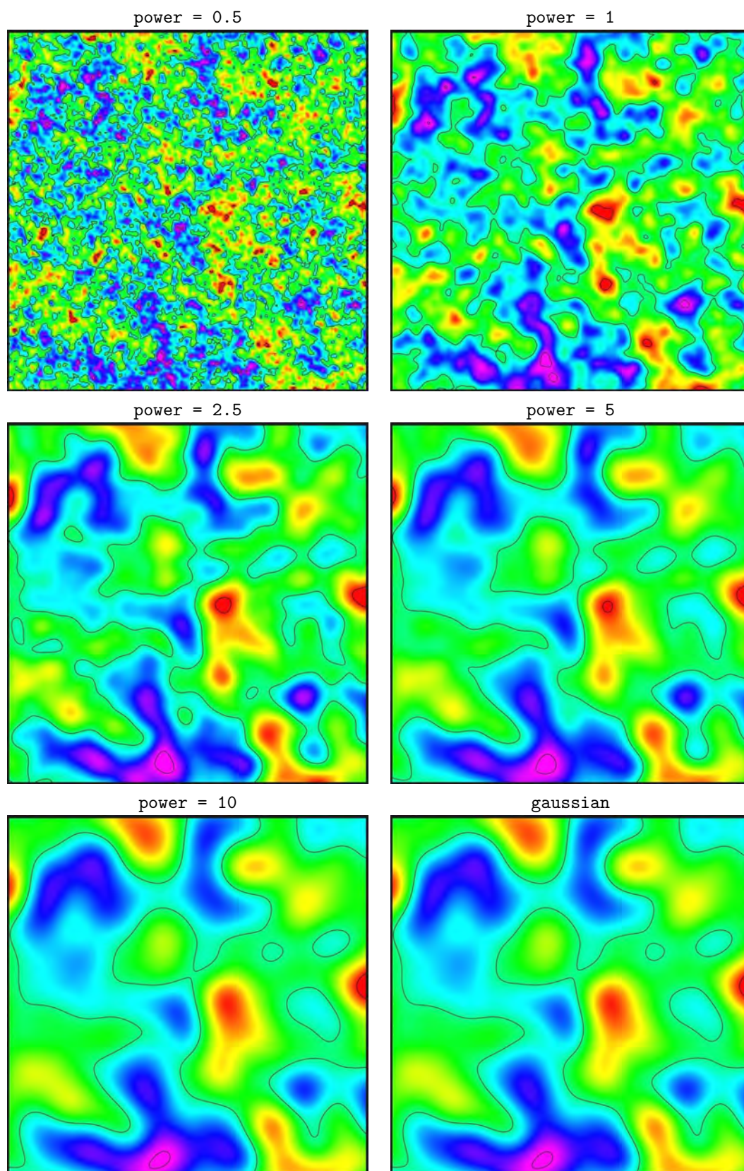
Figure 22.3. Simulated realization using rational quadratic variograms. Note that these variograms approach the gaussian variogram when power becomes large. This variogram is not numerically stable for large values of power so we recommend to use the gaussian variogram instead for power > 10.
