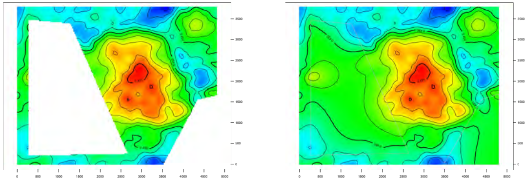
Figure 18.2. Original travel time map to the left with missing areas. Extrapolated travel time map to the right. The default extrapolation method (kriging with 1000 m range) has been used.
