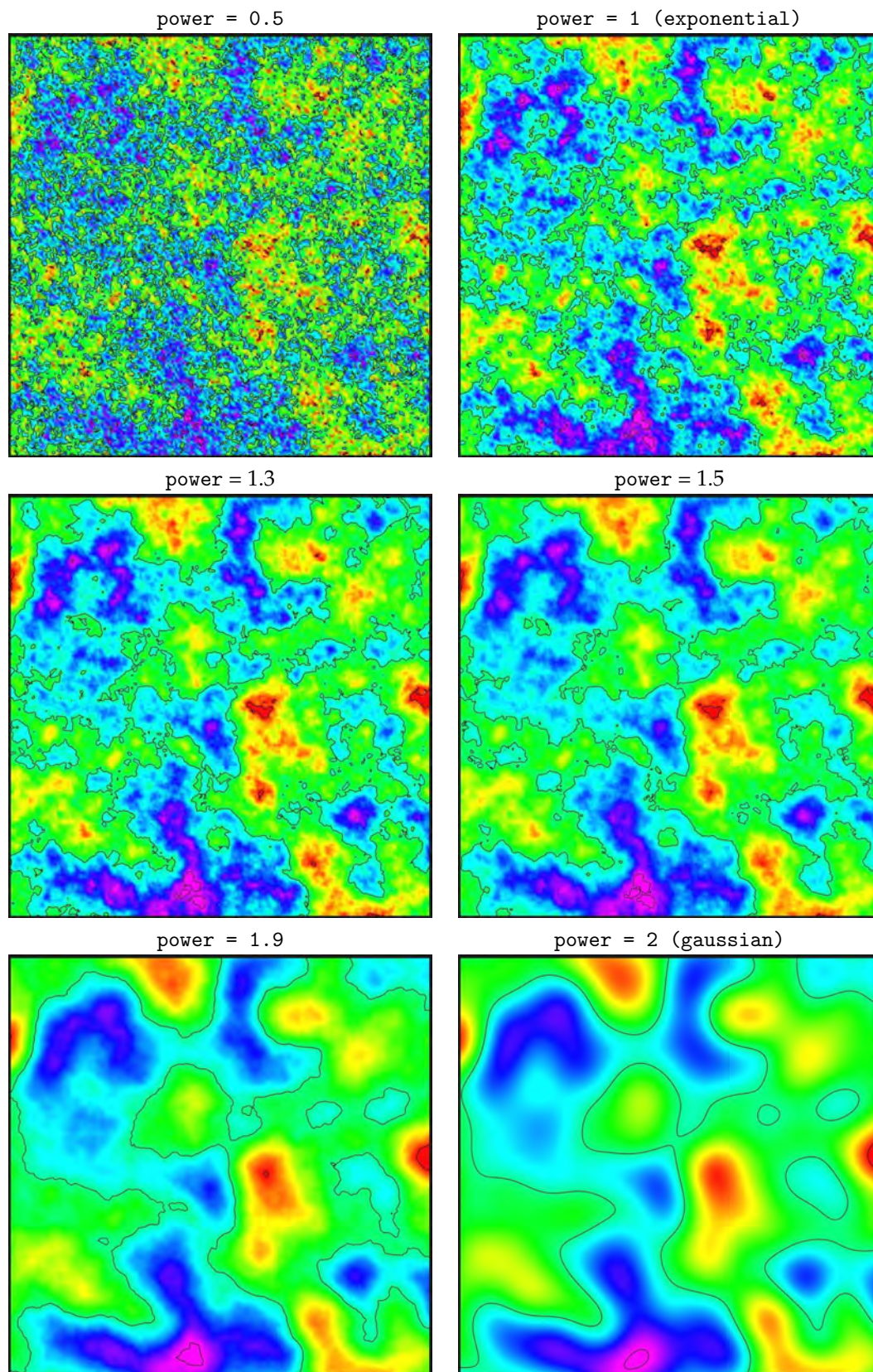
Figure 22.2. Simulated realization using general exponential variograms for different <power> . Note that the exponential variogram is identical to power = 1 and the gaussian variogram is identical to power = 2.
