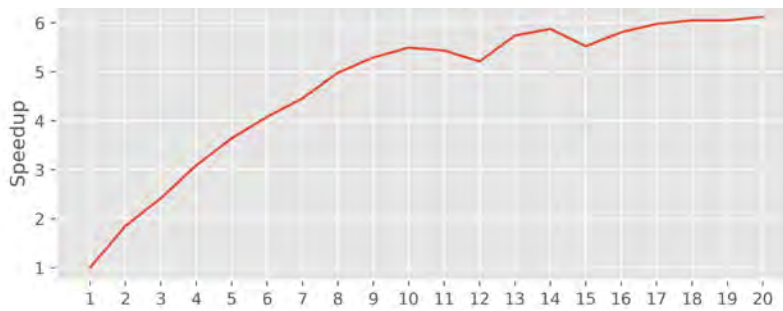
Figure 17.1. Speedup as a function of the number of threads.
