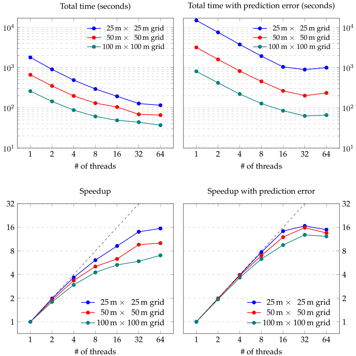
Figure 17.2. Total time and speedup as a function of the number of threads. The three cases are identical but use different grid resolution. The model include 34 predicted surfaces and the surface grids with the finest resolution ( 25\text{ m} \times 25\text{ m} ) contains 1 592 661 grid cells each.
