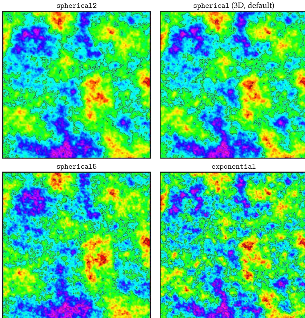
Figure 22.1. Simulated realization using spherical and exponential variograms.
