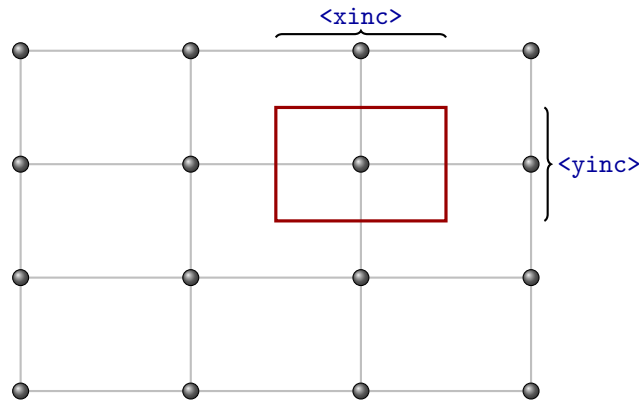
Figure 9.1. The volume within the red rectangle is assigned to the grid node in the center of the red rectangle.
