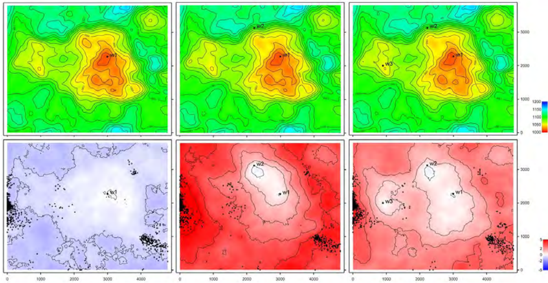
Figure 10.6. At the top are maps of mean surfaces of 1000 realizations with 1 well, 2 wells and 3 wells respectively. They use the same color legend as Figure 10.1 . At the bottom are maps of predicted depths minus the mean surfaces. White color indicates no difference, red color shows that the predicted depths are deeper than the mean, and blue indicates the opposite. The spill points from cases with 1, 2, and 3 wells are included in the lower figures.
