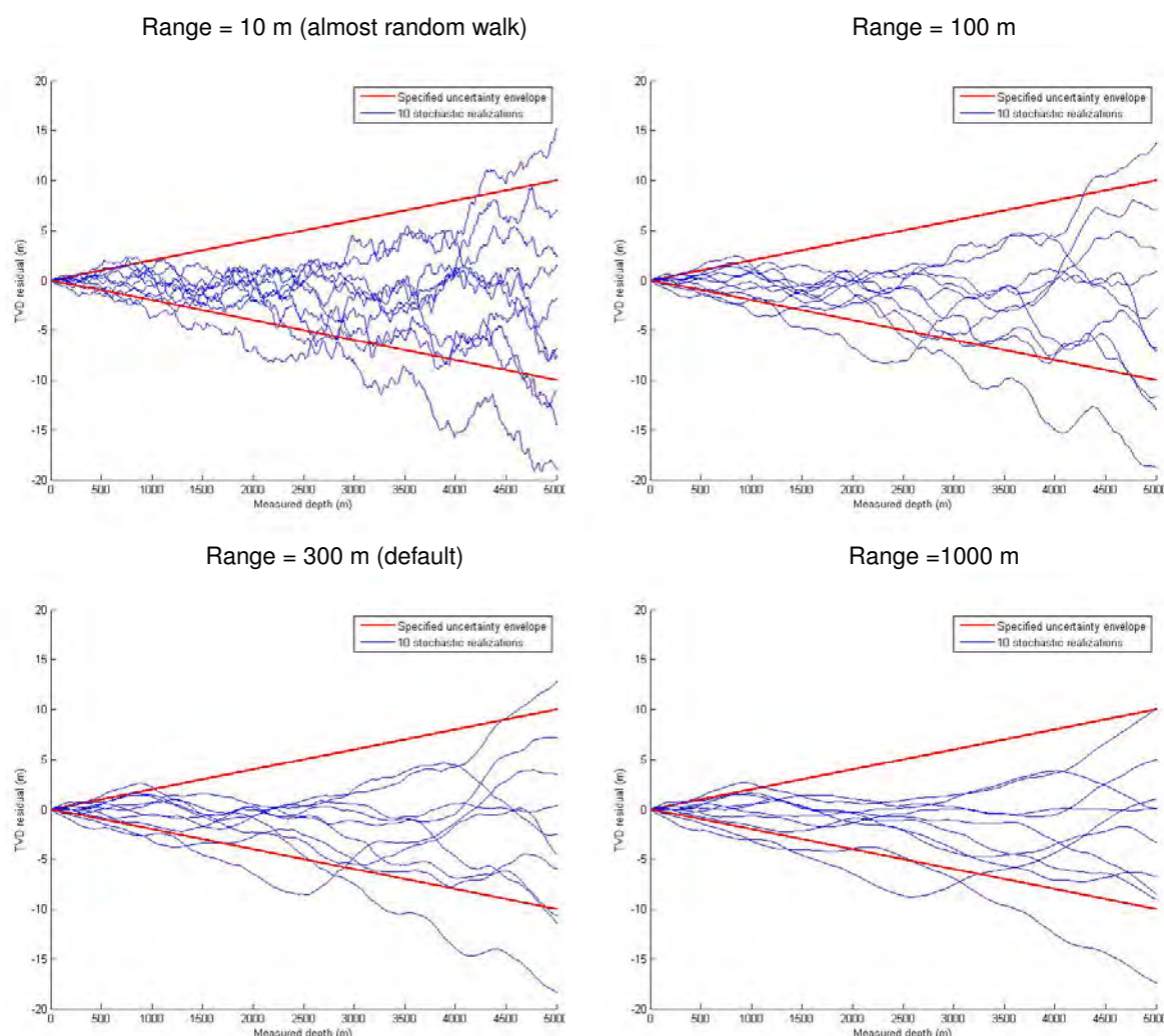
Figure 8.11. Well path TVD uncertainty as a function of WL. The red lines are the TVD uncertainty envelope ( \pm 2SD ) specified by <wellpath-TVD-SD-log-name> . The blue lines are simulated realizations of possible TVD residuals, that is, the difference between the true TVD and the measured TVD. The simulated realizations follow the probability distribution of the integrated Ornstein-Uhlenbeck process. The same random seeds have been used in the four different figures so similar curves with varying smoothness can be recognized in the different figures. The smoothness is specified by <wellpath-TVD-SD-range> .
