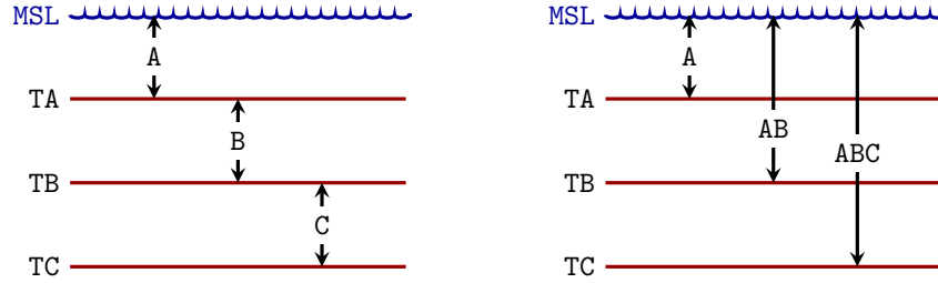
Figure 14.1. Two ways of modeling the surfaces TA, TB, and TC: adding deeper intervals (left) or attaching them directly to the reference surface MSL (right).
