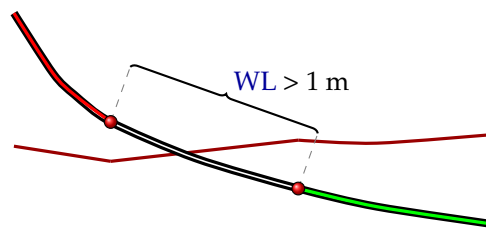
Figure 8.9. Cross section of one surface along a well path. Zonation points (red dots) are added at the edges of the undefined zone log section if the undefined section is long ( \Delta WL > 1 meter). These zonation points may impose necessary surface constraints.
