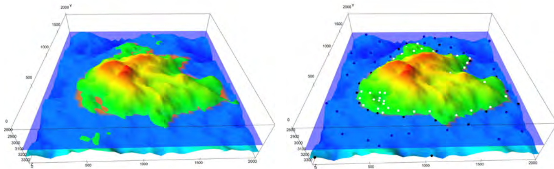
Figure 13.1. Surface constrained by an oil water contact (OWC) . The left figure shows the original surface whereas the right figure shows the surface constrained by the OWC . White points mark sampled locations where the surface is enforced to be above the OWC and black points mark locations where the surface is enforced to be below the OWC .
