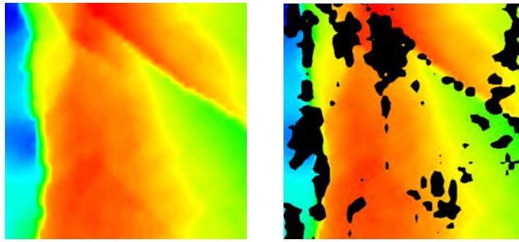
Figure 18.4. Original surface to the left (default). To the right is <set-eroded-nodes-to-undefined> set to yes.
